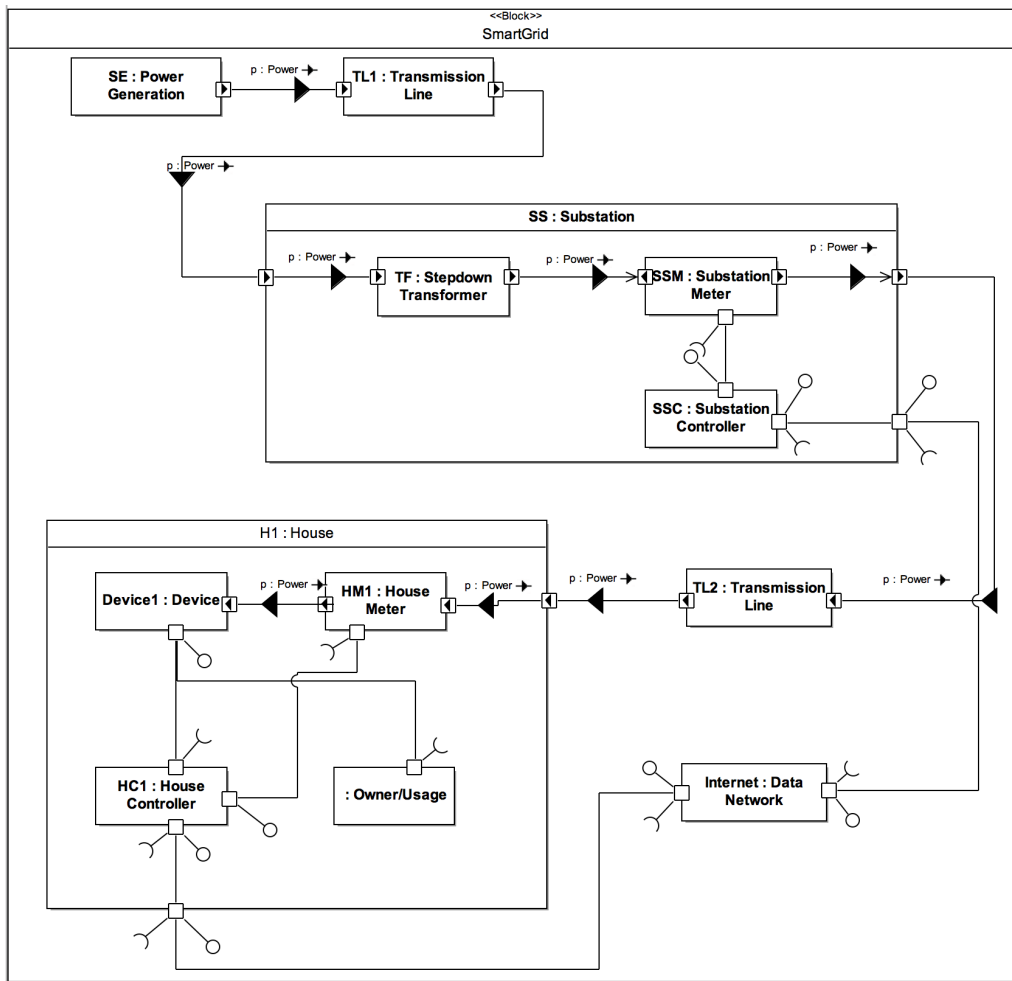
Figure 6.12: Internal Block Diagram of Smart Grid
