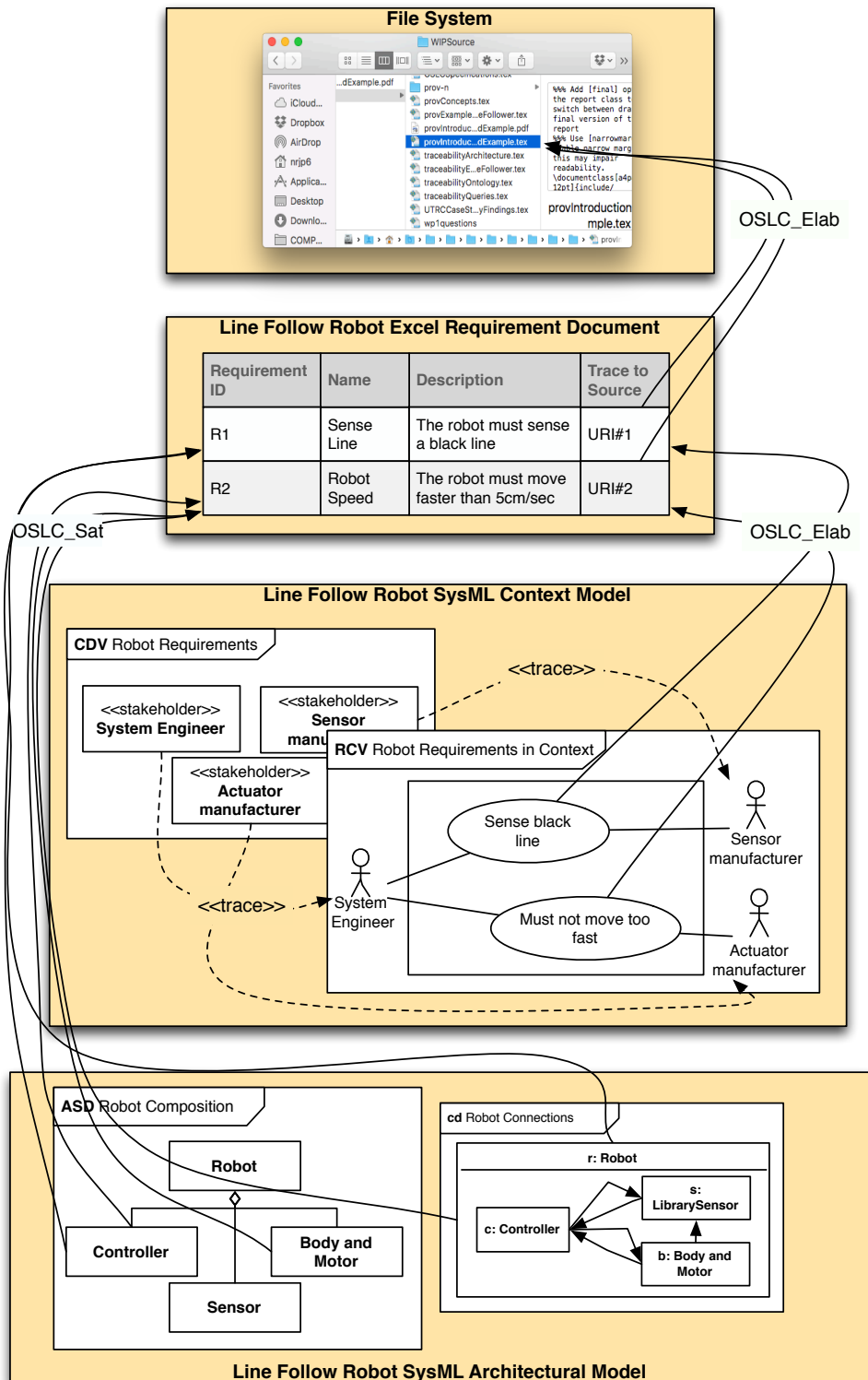
Figure 5.2: Excel and SysML – model overview
